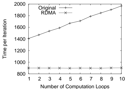
Figure 11. Process Skew Test Results
