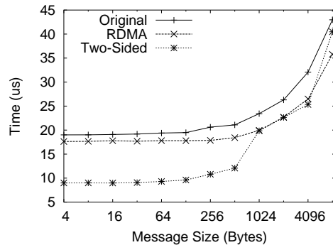
Figure 6. Bi-Directional Latency
