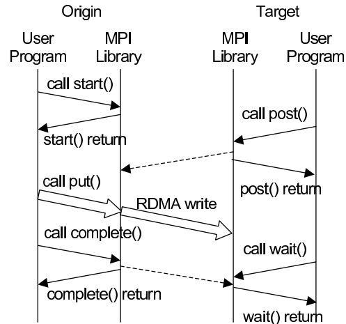
Figure 4. RDMA Based One-Sided Communication Implementation
