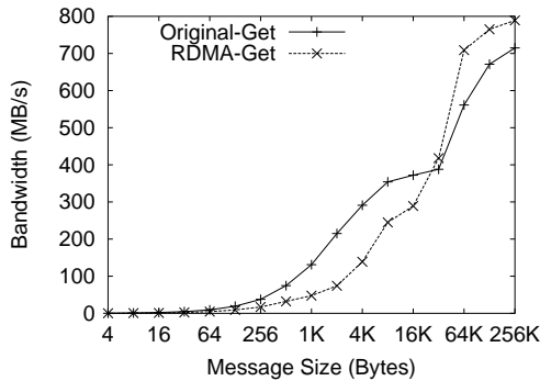
Figure 8. MPI-Get Bandwidth
