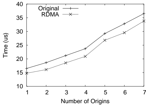
Figure 9. Synchronization Overhead
