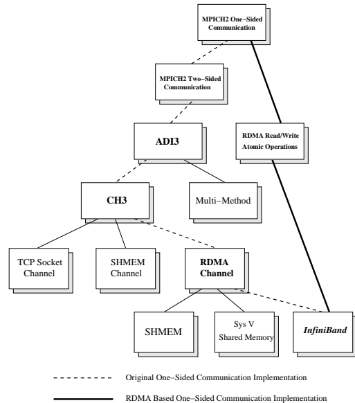
Figure 3. Design Architecture
