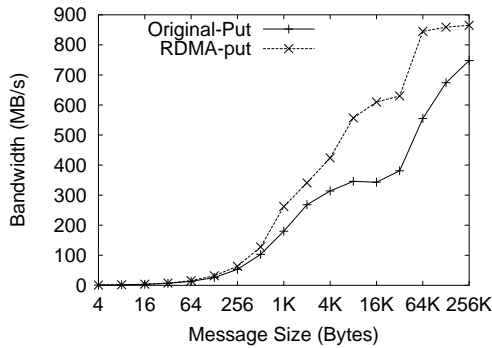
Figure 7. MPI-Put Bandwidth
