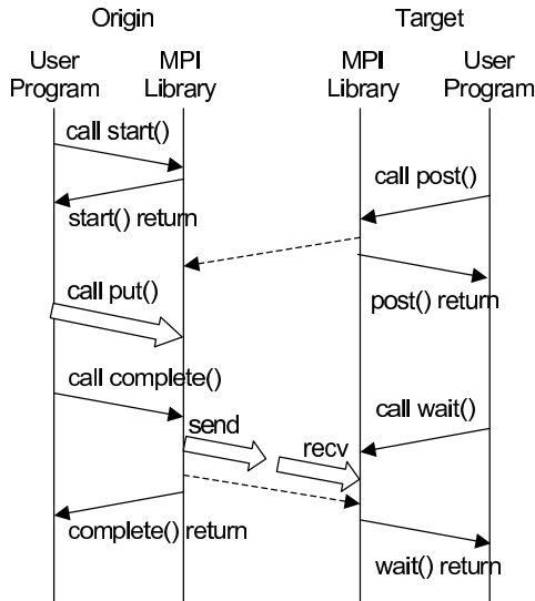
Figure 2. Send/Receive Based One-Sided Communication Implementation
